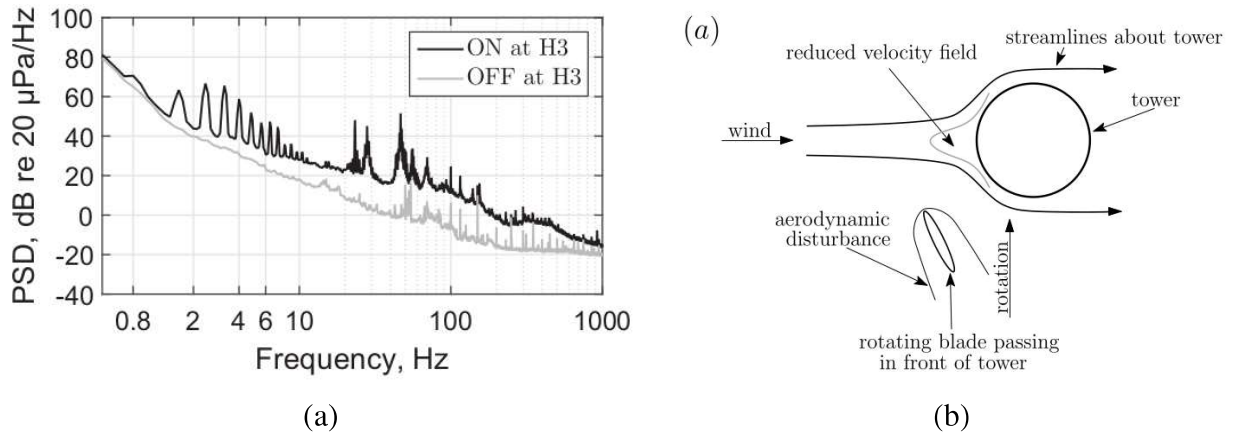
Figure 2: (a) Wind turbine noise spectra measured by Zajamsek et al. (2016) at 3 km from a wind farm, and (b) mechanism of blade-tower interaction noise for an upwind wind turbine (Zajamsek et al. , 2019).
